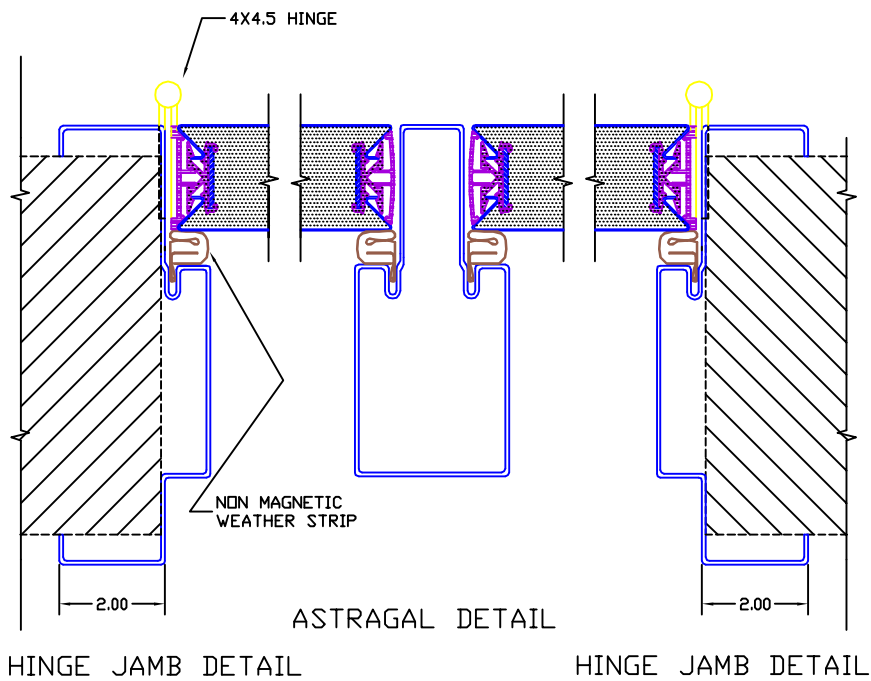
JAMB AND ASTRAGAL DETAIL
