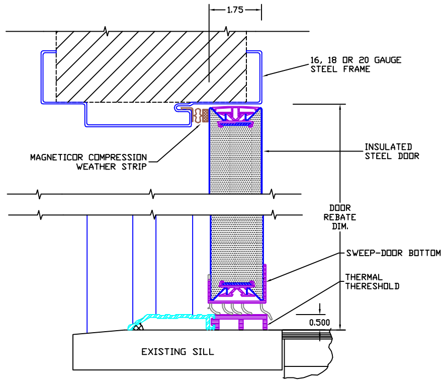
SILL DETAIL
